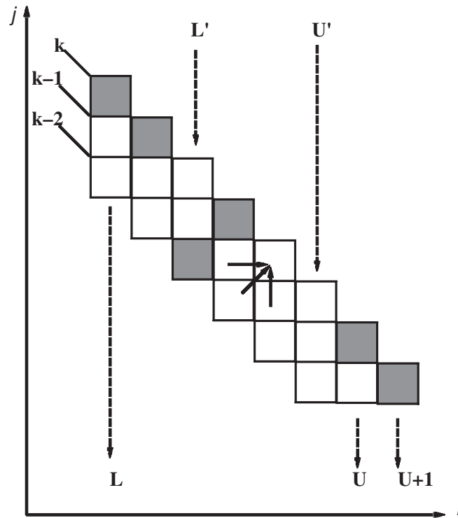
FIG. 1. Pruning of small S -values. The white boxes on antidiagonal k - 1 designate points where S(i, j) > -\infty . S(i, j) on antidiagonal k is computed for i \in [L, U + 1] , after which entries whose scores are too small are reset to -\infty , and any such positions at the ends of the white boxes are pruned away giving L' and U' .
